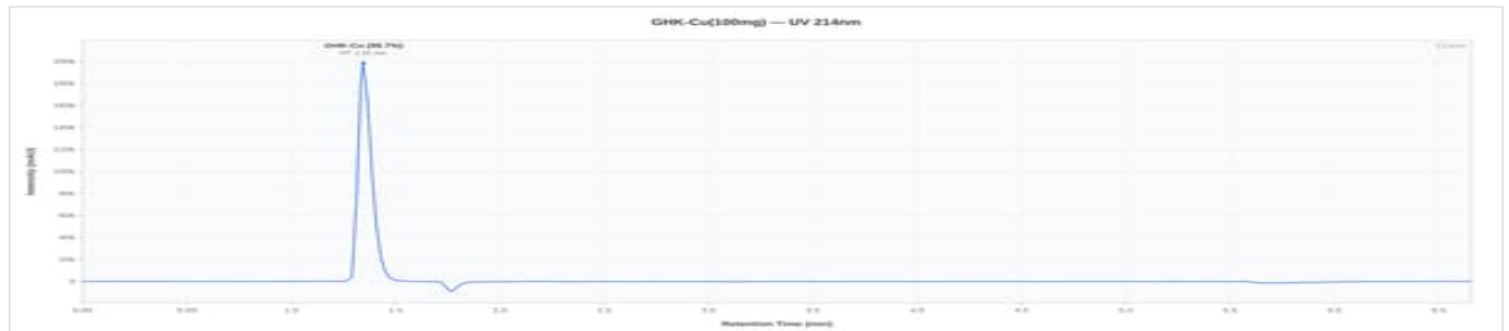
GHK-Cu 100mg - AEYGHK100-01: UV Chromatogram
